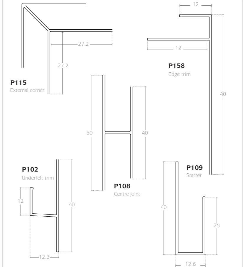
Cladding trims
