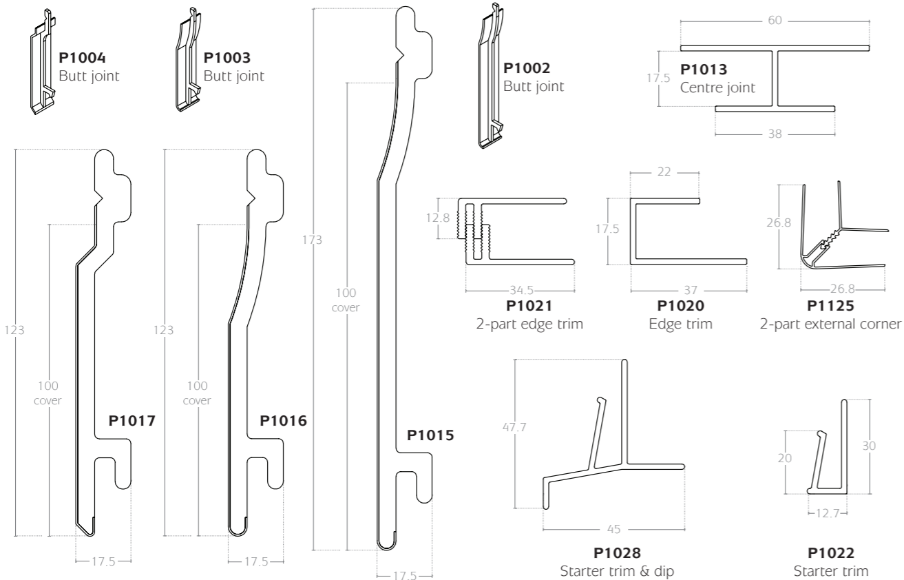
Foam cladding
