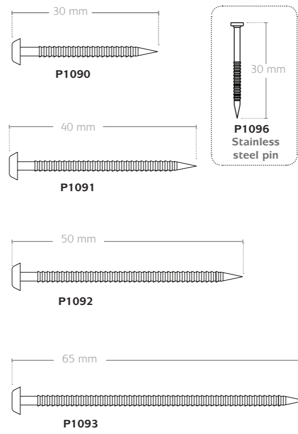
PVC headed pins and stainless steel pin
